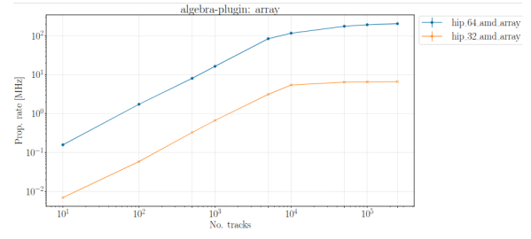
Figure 19: Throughput Comparison of HIP on AMD : Single precision vs Double precision
