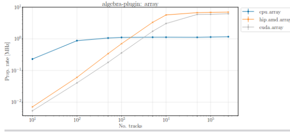
Figure 15: Throughput Comparison of HIP (AMD) & CUDA (NVIDIA) & CPU
