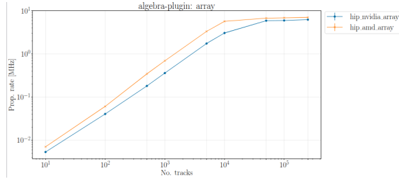
Figure 17: Throughput Comparison of HIP (AMD) & HIP (NVIDIA)
