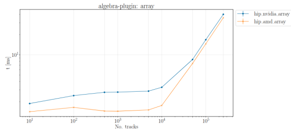
Figure 18: Latency Comparison of HIP (AMD) & HIP (NVIDIA)
