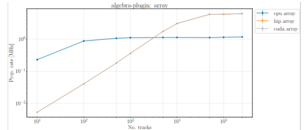
Figure 13: Throughput Comparison of HIP & CUDA & CPU performance on NVIDIA Backends
